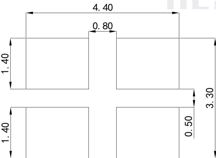
Fig.1-5 Soldering patterns 推荐焊盘
