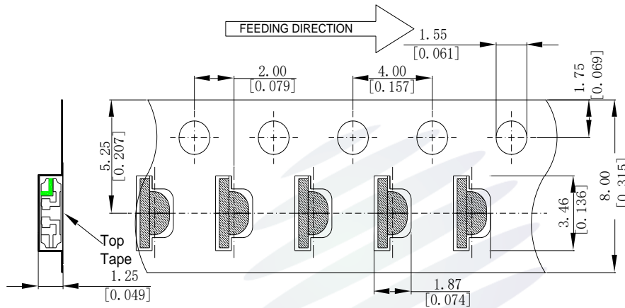
Fig.2-1 Carrier Tape Dimension 载带尺寸
