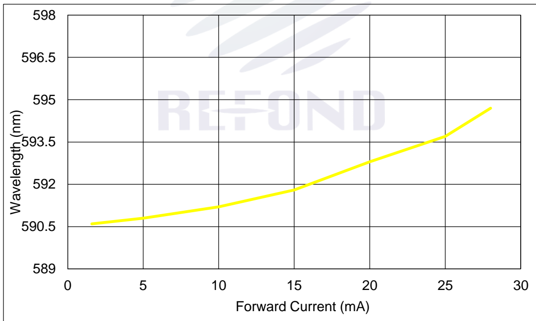
Fig.1-11 Forward Current Vs Dominate Wavelength (Ta=25°C) 正向电流与主波长关系曲线 (黄光)
