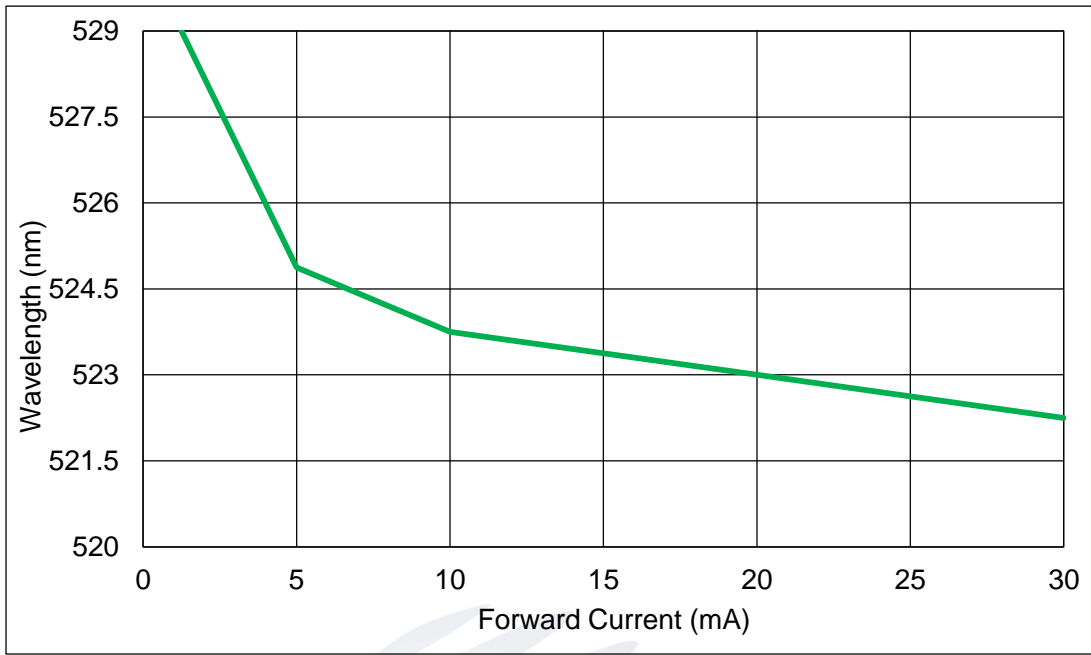
Fig.1-10 Forward Current Vs Dominate Wavelength (Ta=25°C) 正向电流与主波长关系曲线 (绿光)
