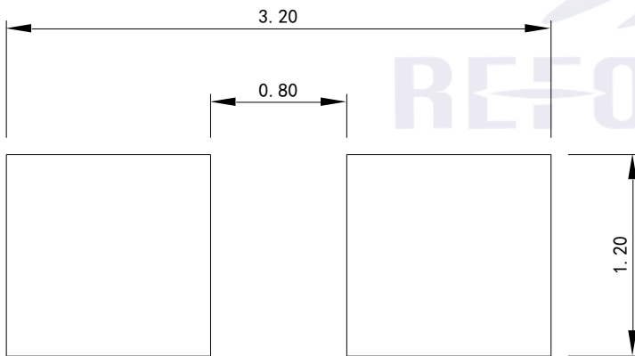
Fig.1-5 Soldering patterns 推荐焊盘
