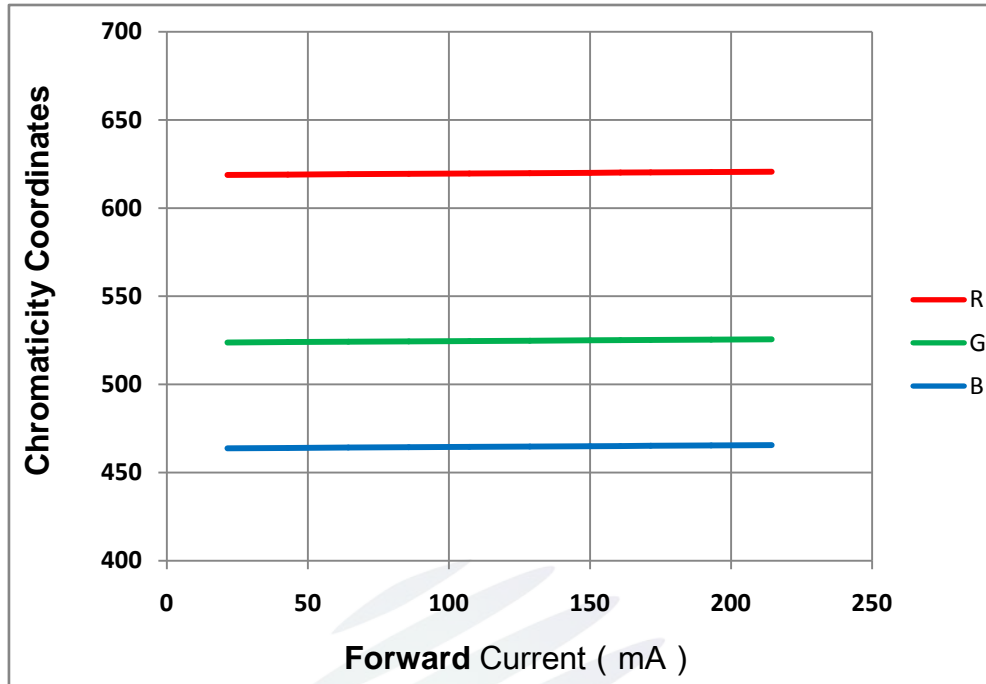
Fig. 1-13 Forward current Vs Dominate wavelength正向电流特性与主波长曲线
