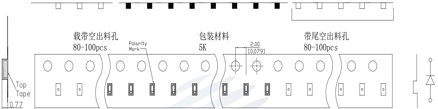
Fig.2-1 Carrier Tape Dimension 载带尺寸
