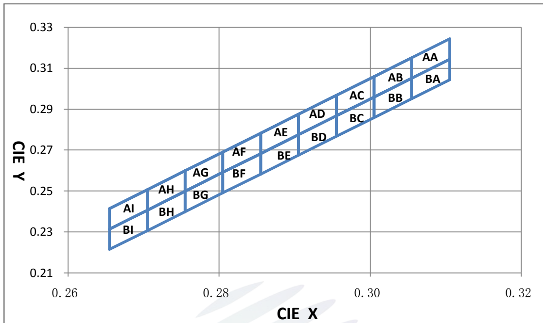
Fig. 1-6 The C.I.E Chromaticity Diagram CIE色度图
