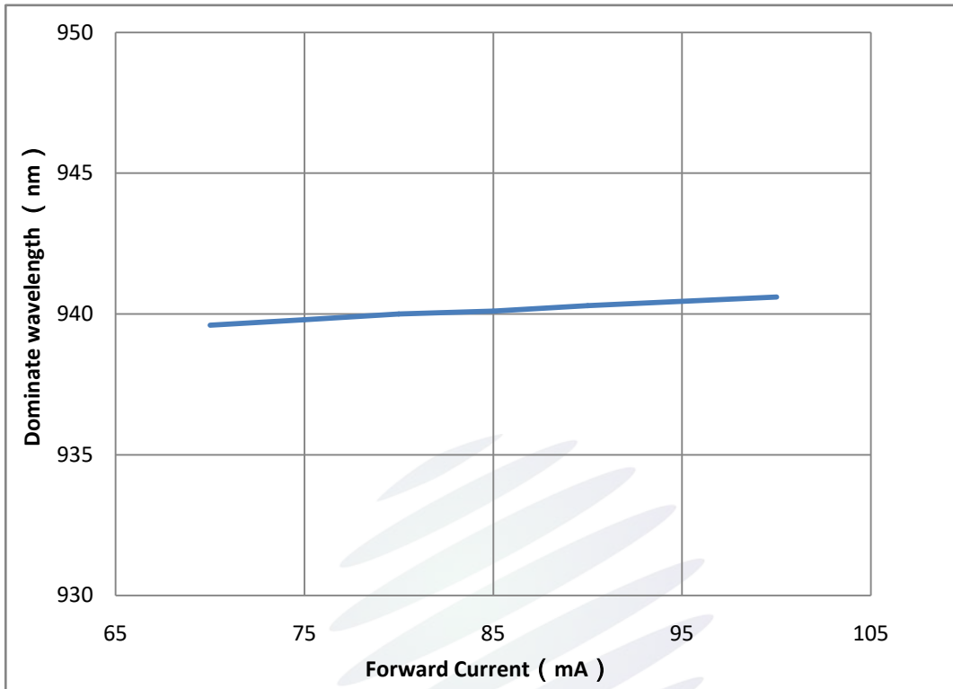
Fig. 1-13 Forward current vs. Dominate wavelength (Ts=25°C)正向电流与主导波长特性曲线(Ts=25°C)
