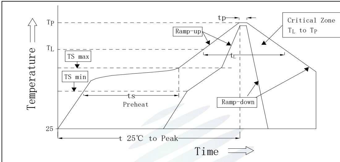
Fig.3-1SMT Reflow Soldering Instructions SMT 回流焊说明
