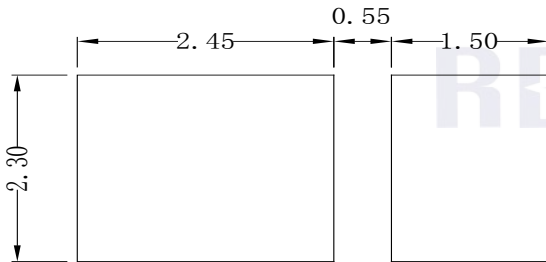
Fig.1-5 Soldering Patterns 推荐焊盘
