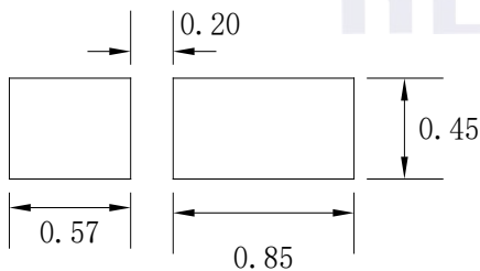
Fig. 1-5 Soldering Patterns 推荐焊盘
