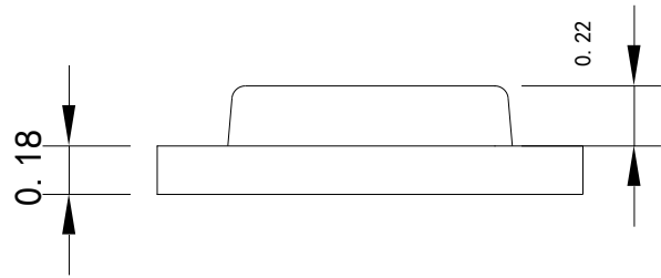
Fig.1-2 Side view 侧面视图
