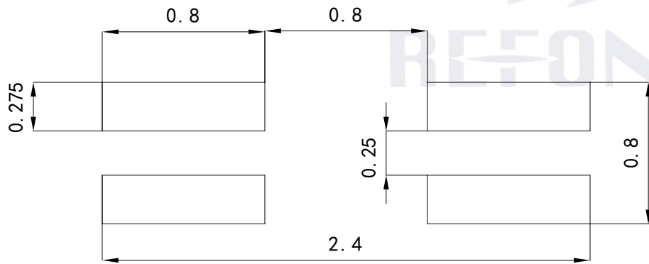
Fig.1-5 Soldering patterns 推荐焊盘
