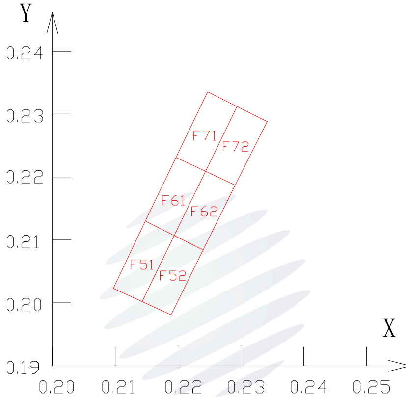
Fig. 1-6 The C.I.E Chromaticity Diagram CIE色度图
