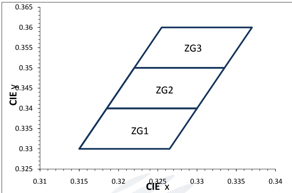
Fig. 1-6 The C.I.E Chromaticity Diagram CIE色度图
