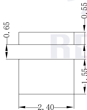
Fig.1-5 Soldering Patterns 推荐焊盘
